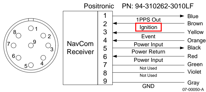
Ignition Pin
