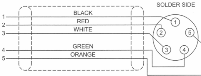
Figure D1: Event Cable Wiring Diagram
