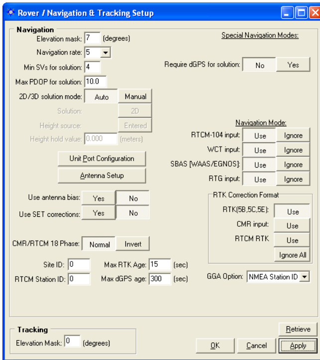
Figure 16: StarUtil Rover Navigation Setup
