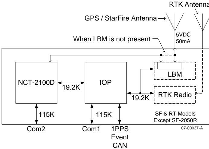
Figure 11: SF-2050G/M Block Diagram
