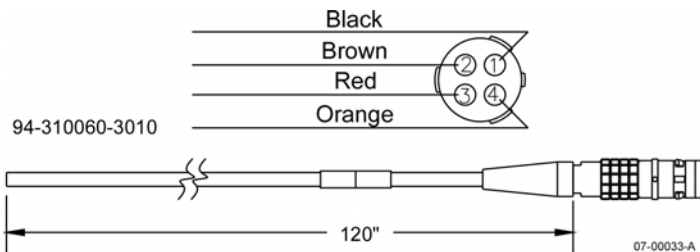
Figure 4: Optional DC Power Cable
