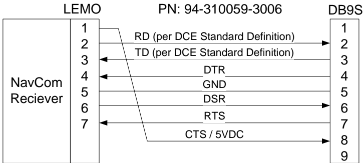
Figure 6: NavCom Serial Cable P/N 94-310059-3006 Connect pin 5 to shield of cable at both ends.
